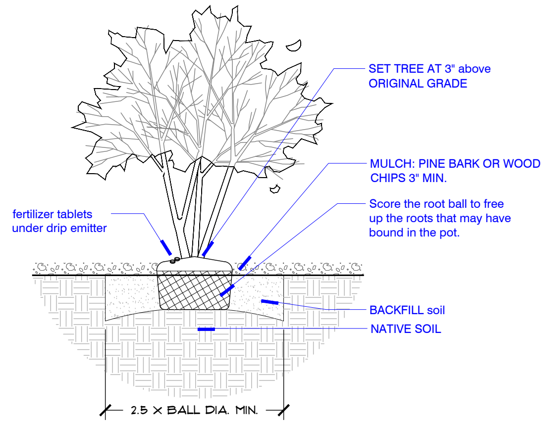
2 DECIDUOUS MULTI-STEM TREE PLANTING 1" = 1'-0"
