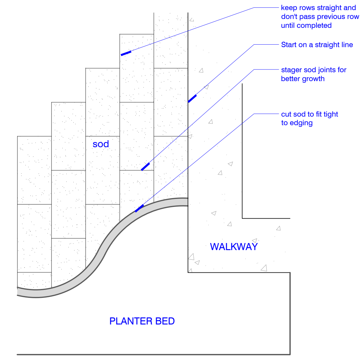
4 SOD LAYING PATTERN 1" = 1'-0"
