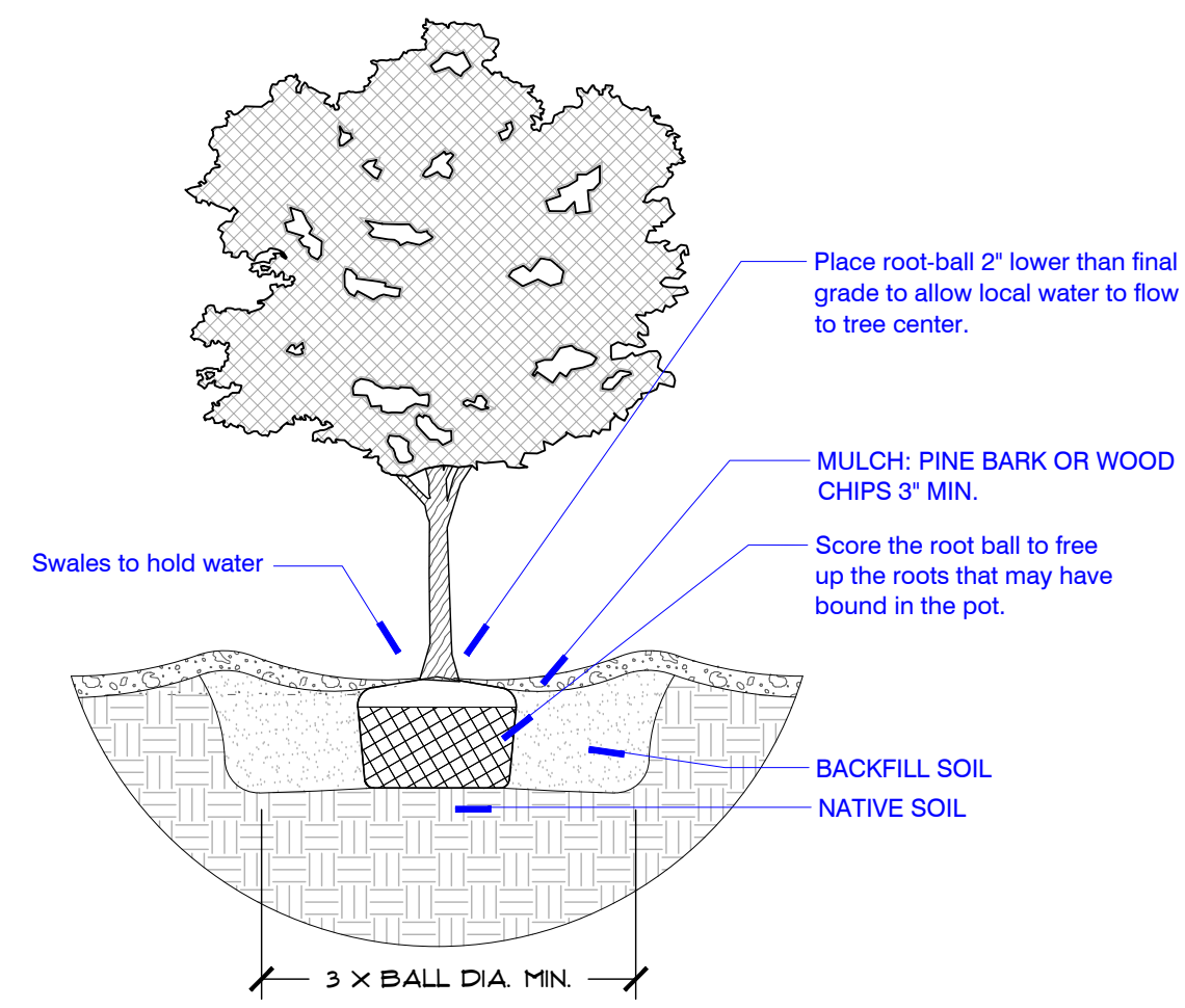
1 DECIDUOUS TREE PLANTING 1" = 1'-0"
